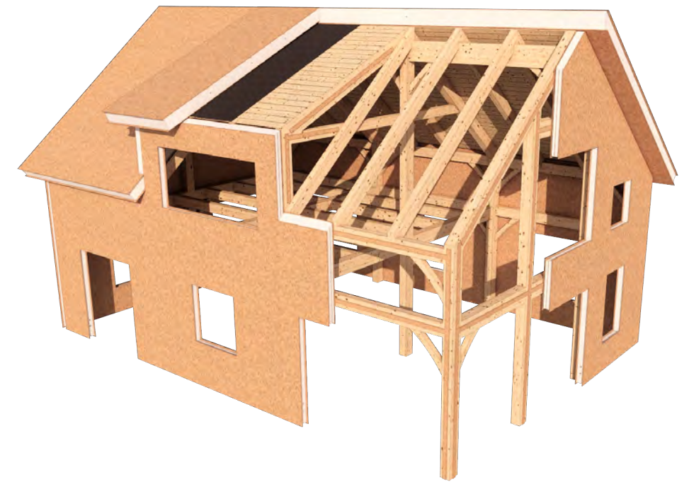
STEP 6. Roof SIPs
