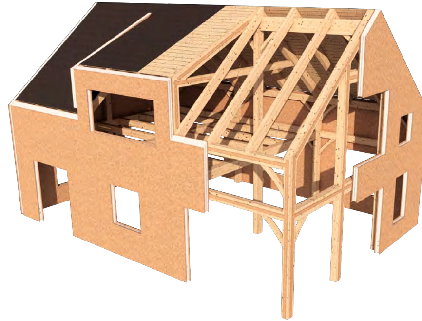
STEP 5. Wall SIPs
